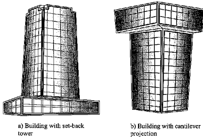
Figure 23 Buildings with vertical setbacks
