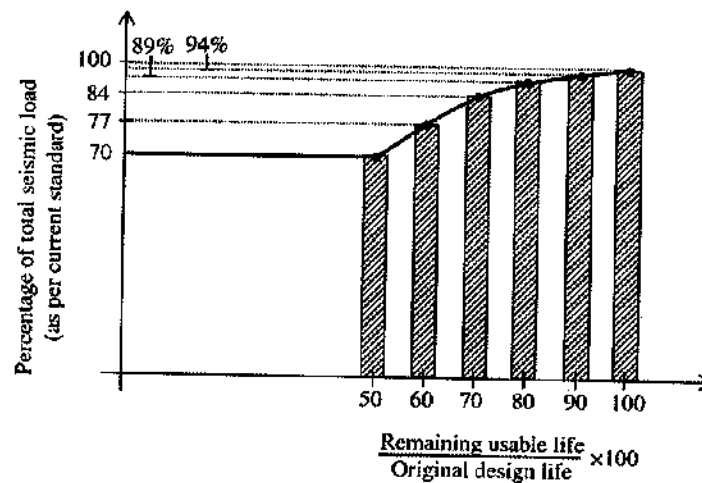
Figure 47 Design seismic load as a function of remaining usable life
