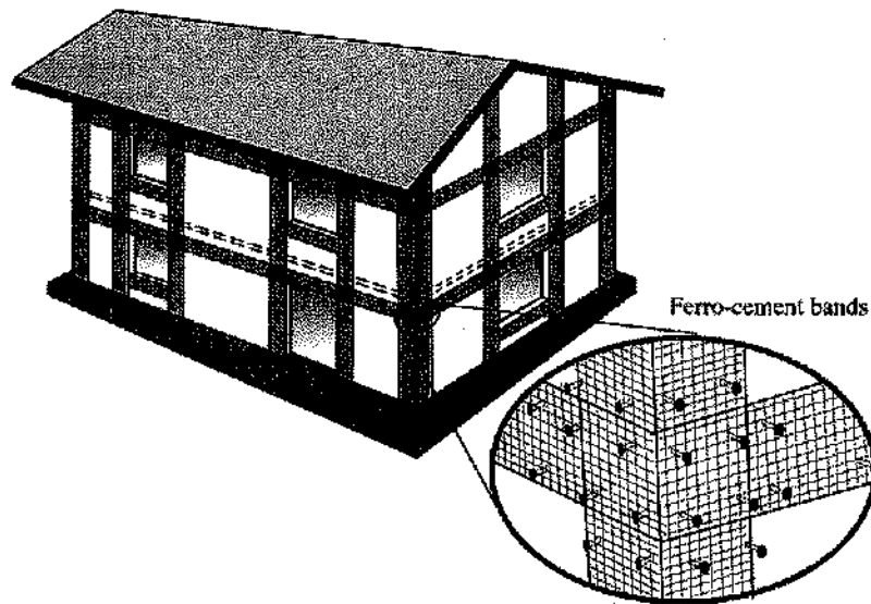
Figure 54 Splint and bandage strengthening technique (IS 13935)
