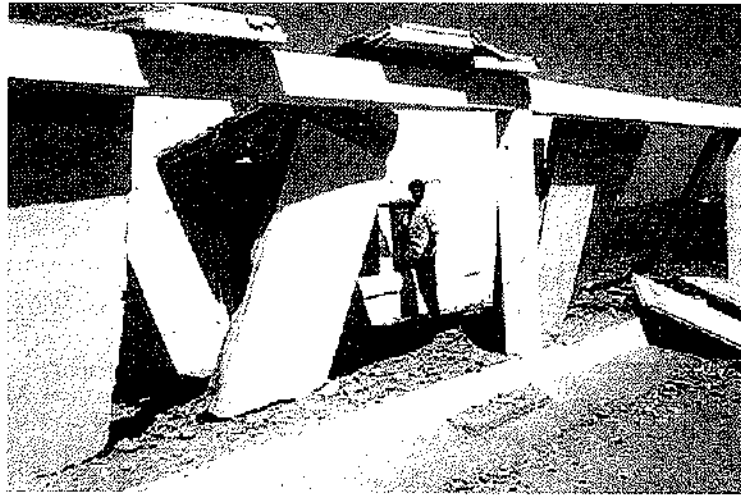
Figure 43 Lack of proper connection in a pre-cast building (after Bhuj earthquake, 2001) (Source: www.nicee.org )
