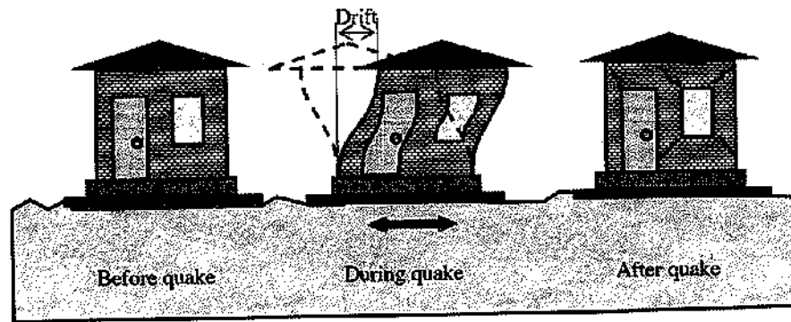
Figure 11 Elastic behaviour of a building (Murty, 2005)
