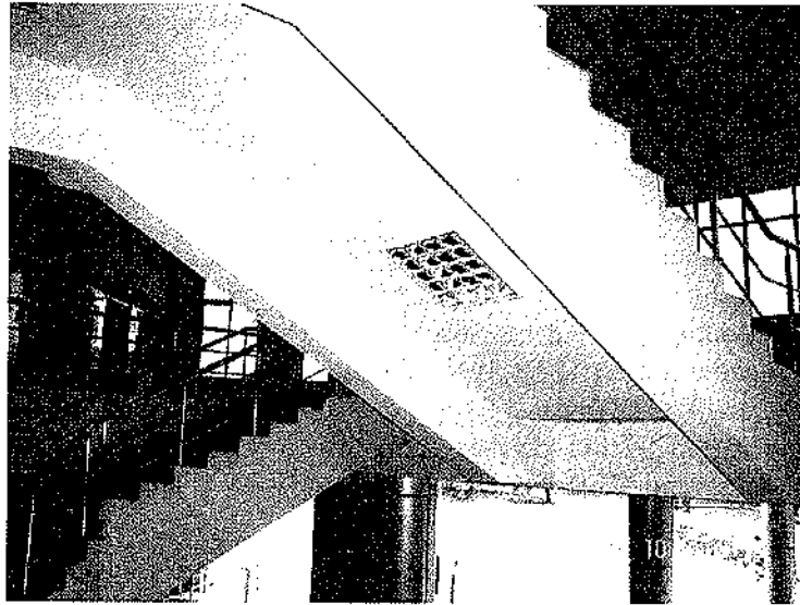
Figure 42 Stairs with stringer beams connected to the building frame
